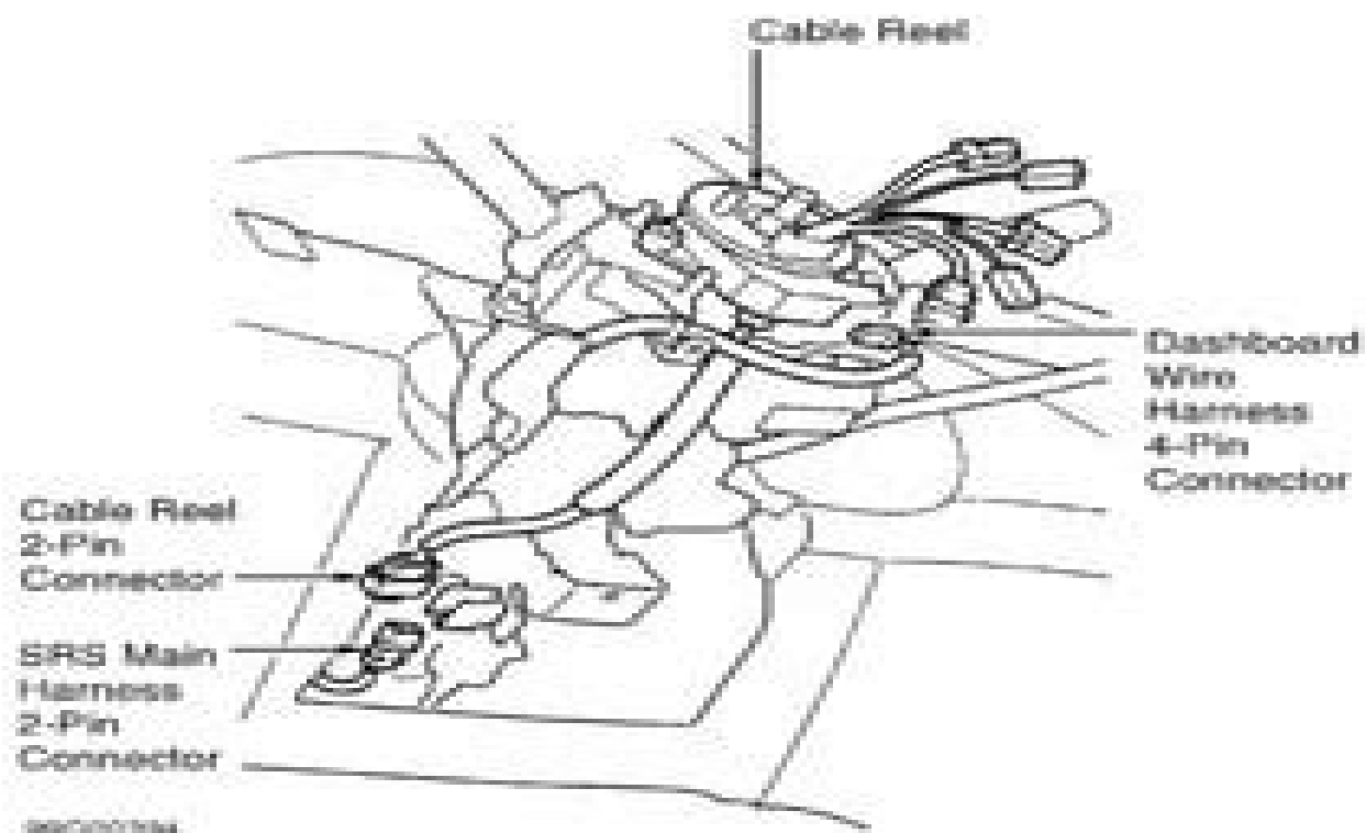
Fig. 11: Identifying Cable Reel Courtesy of AMERICAN HONDA MOTOR CO., INC.
