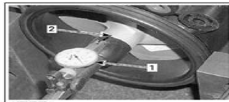
TYPICAL — MEASURING IMPELLER SHAFT RADIAL PLAY 1. Dial gauge 2. Measure close to impeller hub end
