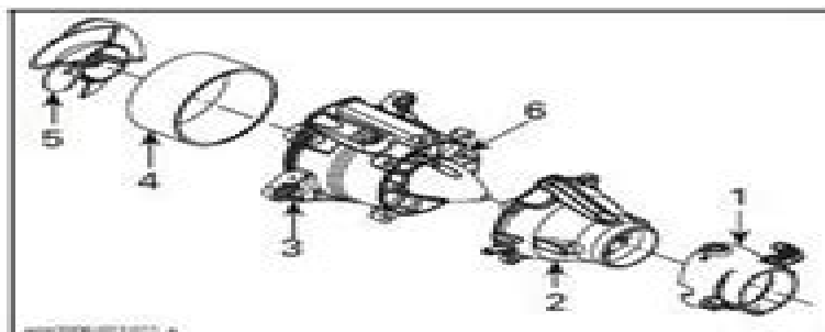
TYPICAL 1. Nozzle 2. Venturi 3. Jet pump housing 4. Wear ring 5. Impeller 6. Stator
