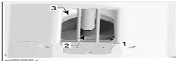
TYPICAL — UNDERNEATH HULL 1. Impeller 2. Impeller boot 3. Wear ring
