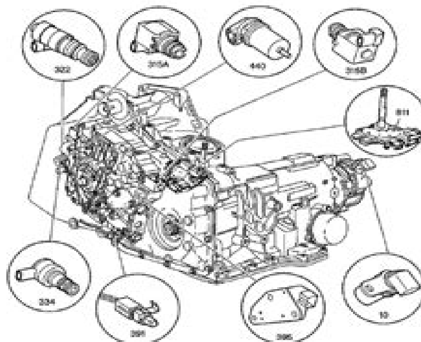
Fig. 4: Automatic Transmission Internal Electronic Component Locations Courtesy of GENERAL MOTORS CORP.
