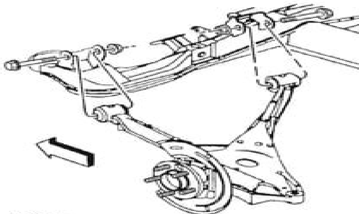
Fig. 4: Removing/Installing Lower Control Arm Mounting Bolts & Nuts Courtesy of GENERAL MOTORS CORP.
