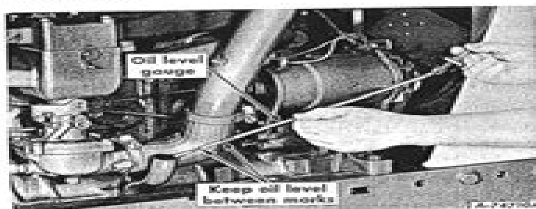
Illustr. 8 Crankcase oil level gauge. (gasoline and LP Gas engines).
