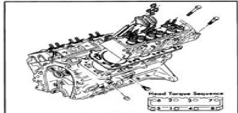
Figure 16 Cylinder Head Installation
