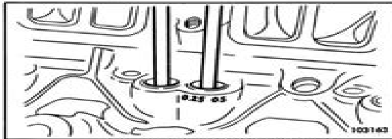
Figure 15 Oversize Lifter Marking
