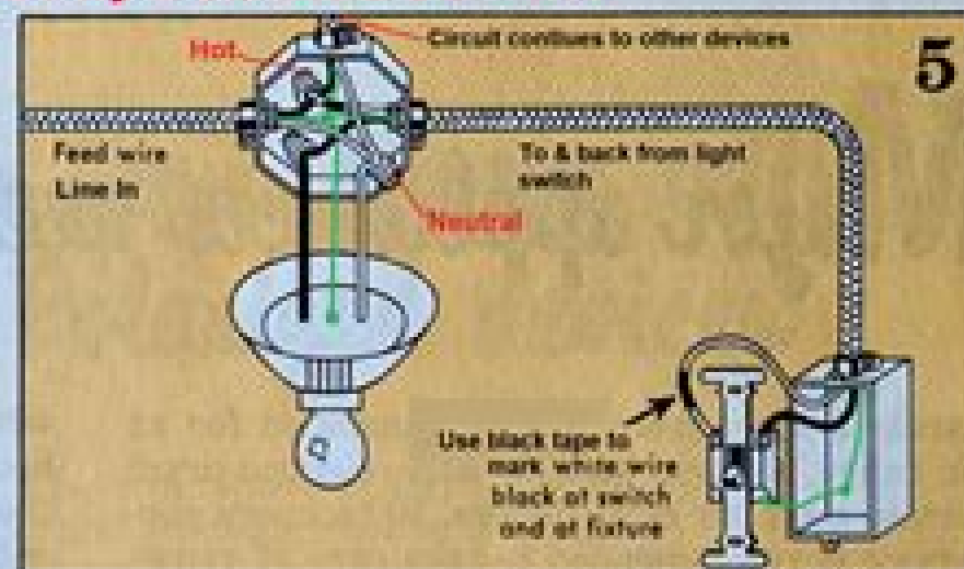
To add wall switch to control ceiling light in middle of run
