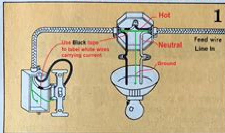
To add a wall switch to control ceiling light at end of run
