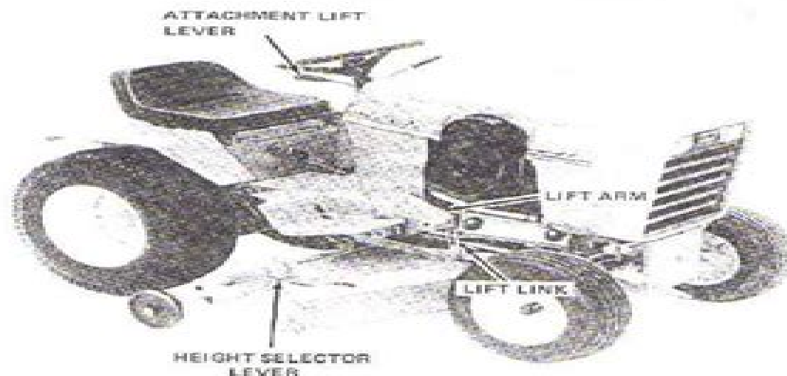
FIGURE 1 OPERATION
