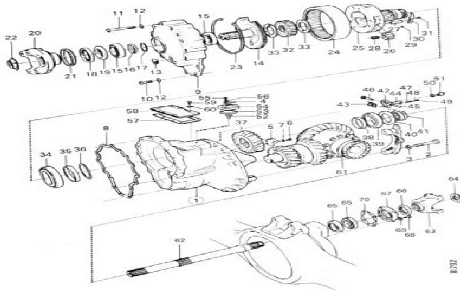
Axle gear RBP831, planetary gear
