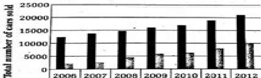
Data regarding number of cars sold during 7 years
