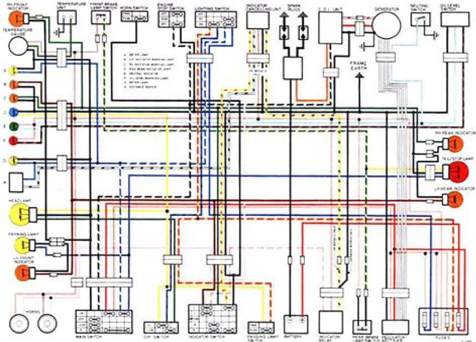
Wiring diagram - RD250 and 350 LC models
