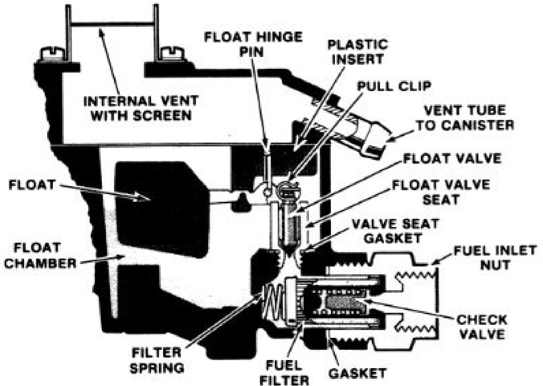
FLOAT SYSTEM
