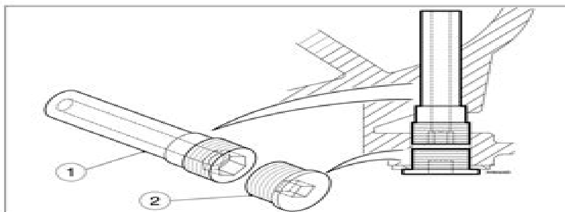
18.14b Transmission fluid drain plug (1) and oil level plug (2) – from RPO no. 09857
