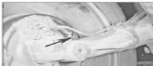
19.2a Prise the grommet (arrowed) from the rear drum brake backplate
