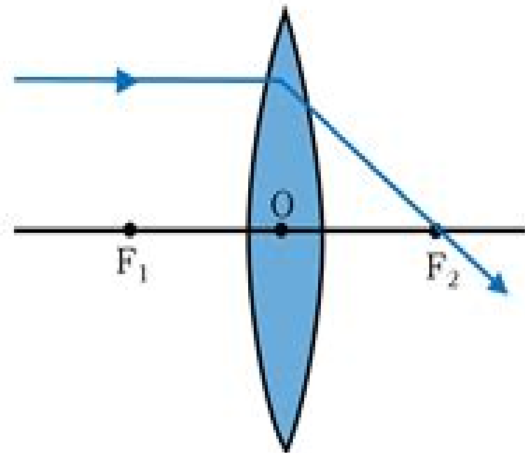
Convex Lens
