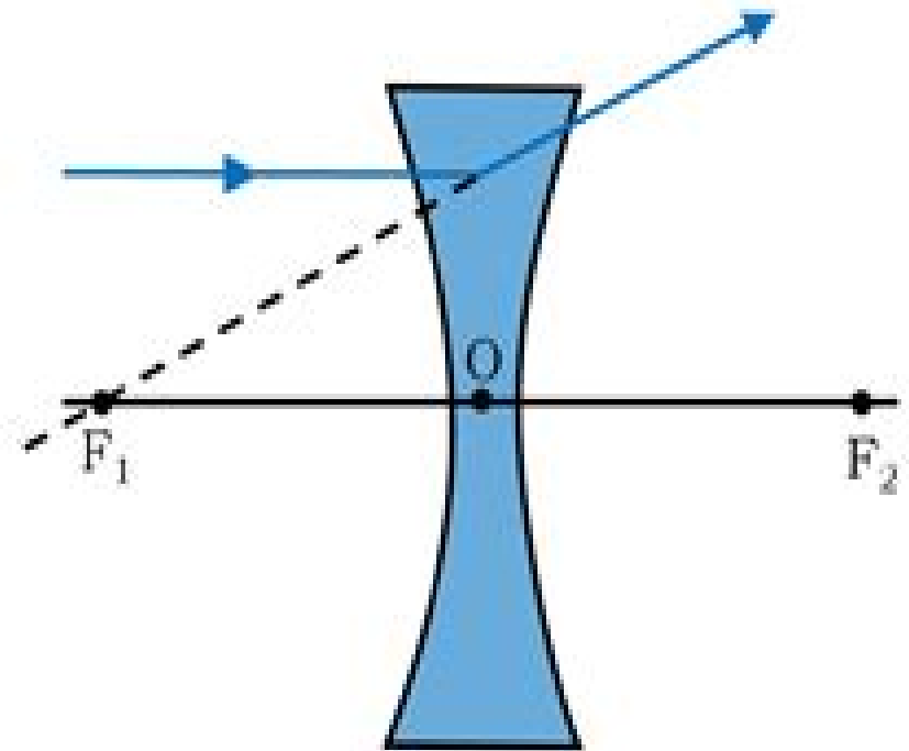
Concave Lens
