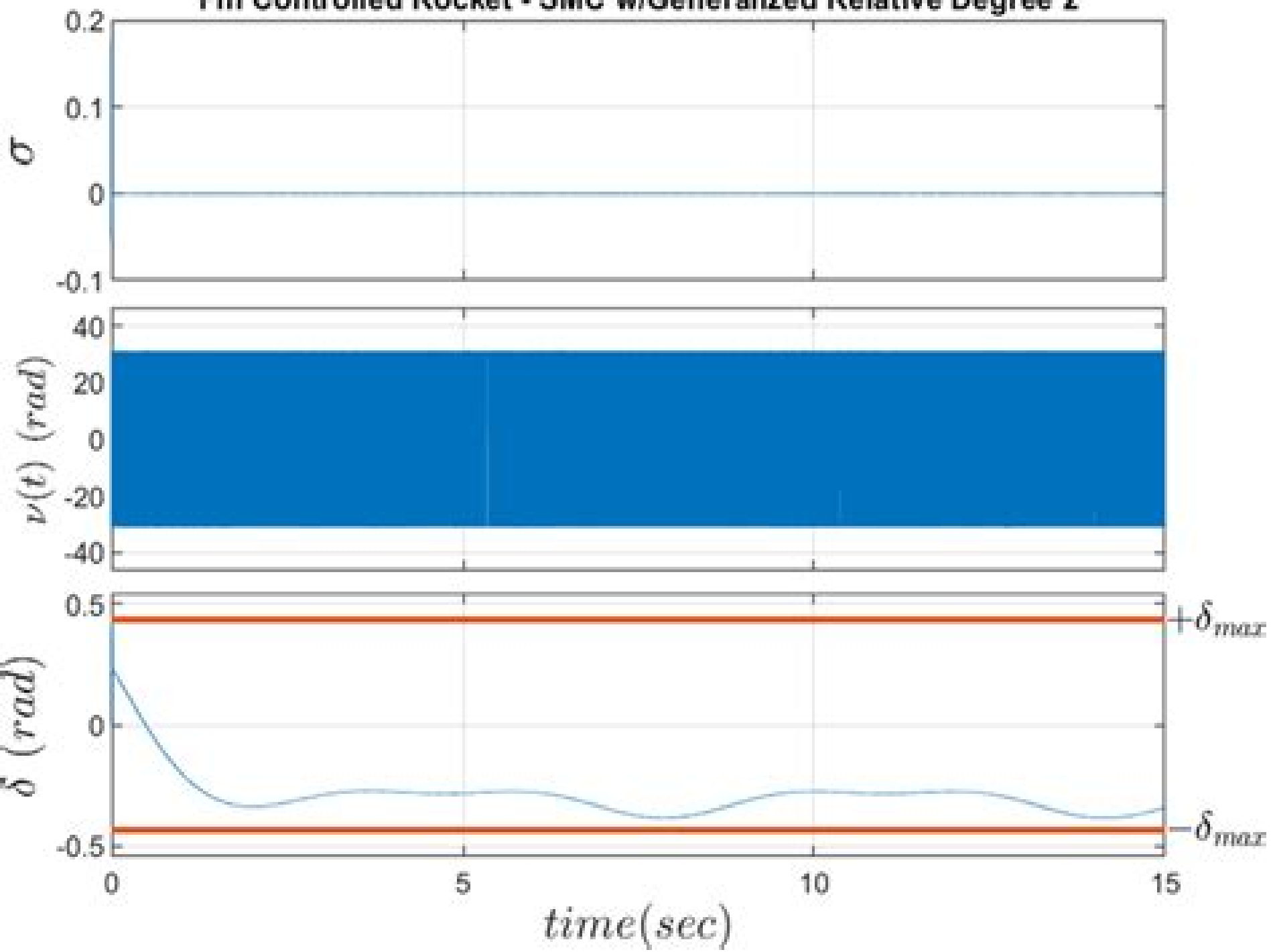
Fin Controlled Rocket - SMC w/Generalized Relative Degree 2
