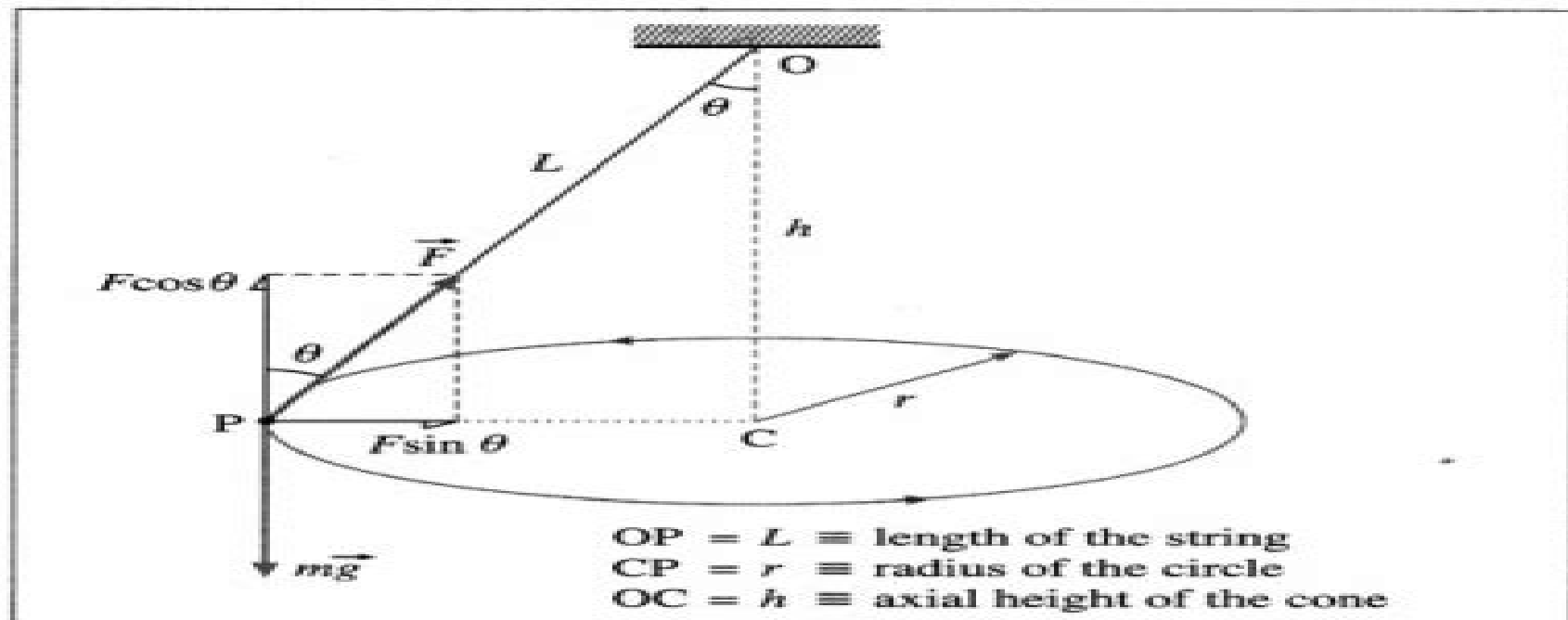
Fig. 1.16 : Conical pendulum
