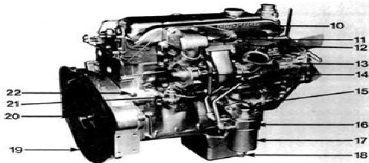
VIEW OF CAMSHAFT SIDE OF T4.236 ENGINE
