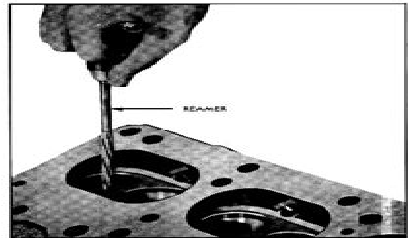
Fig. 6-47 Fitting Valve Stems to Guide
