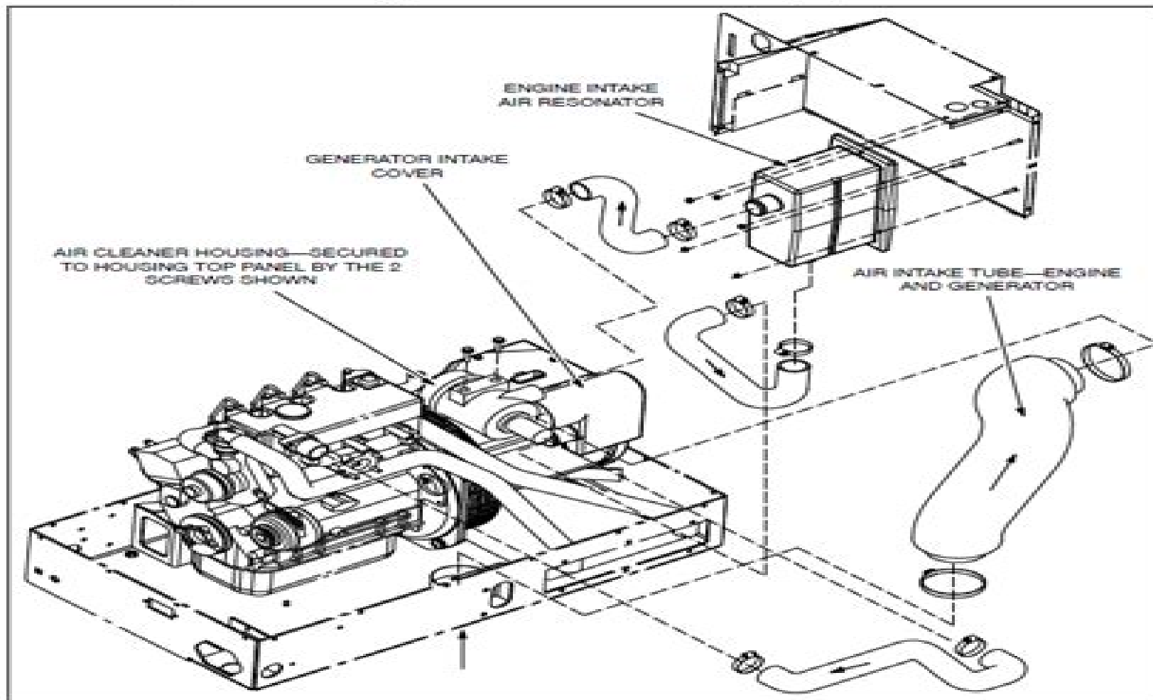
FIGURE 6-1. AIR INTAKE COMPONENTS (BEGINNING SPEC C)
