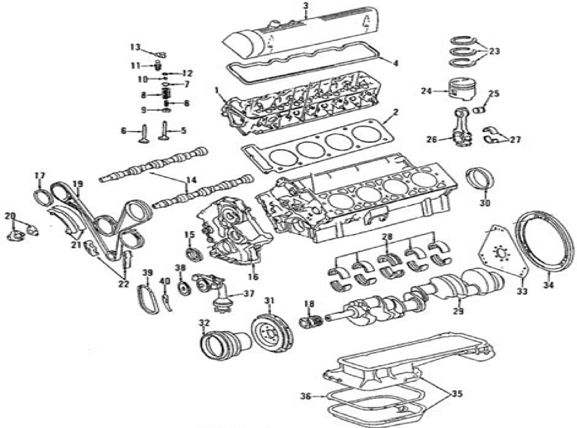
ENGINE - 8 CYLINDER
