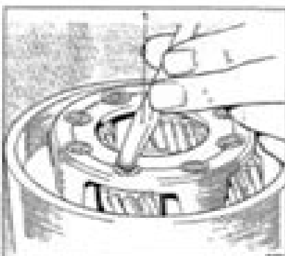
Fig. 11B-14 Inspecting a piston pin 1. Check
