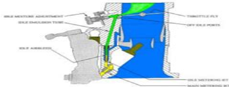
FIGURE 1. TYPICAL IDLING SYSTEM IN A FLOAT CARBURETOR.
