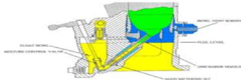
FIGURE 1. TYPICAL IDLING SYSTEM IN A FLOAT CARBURETOR.
