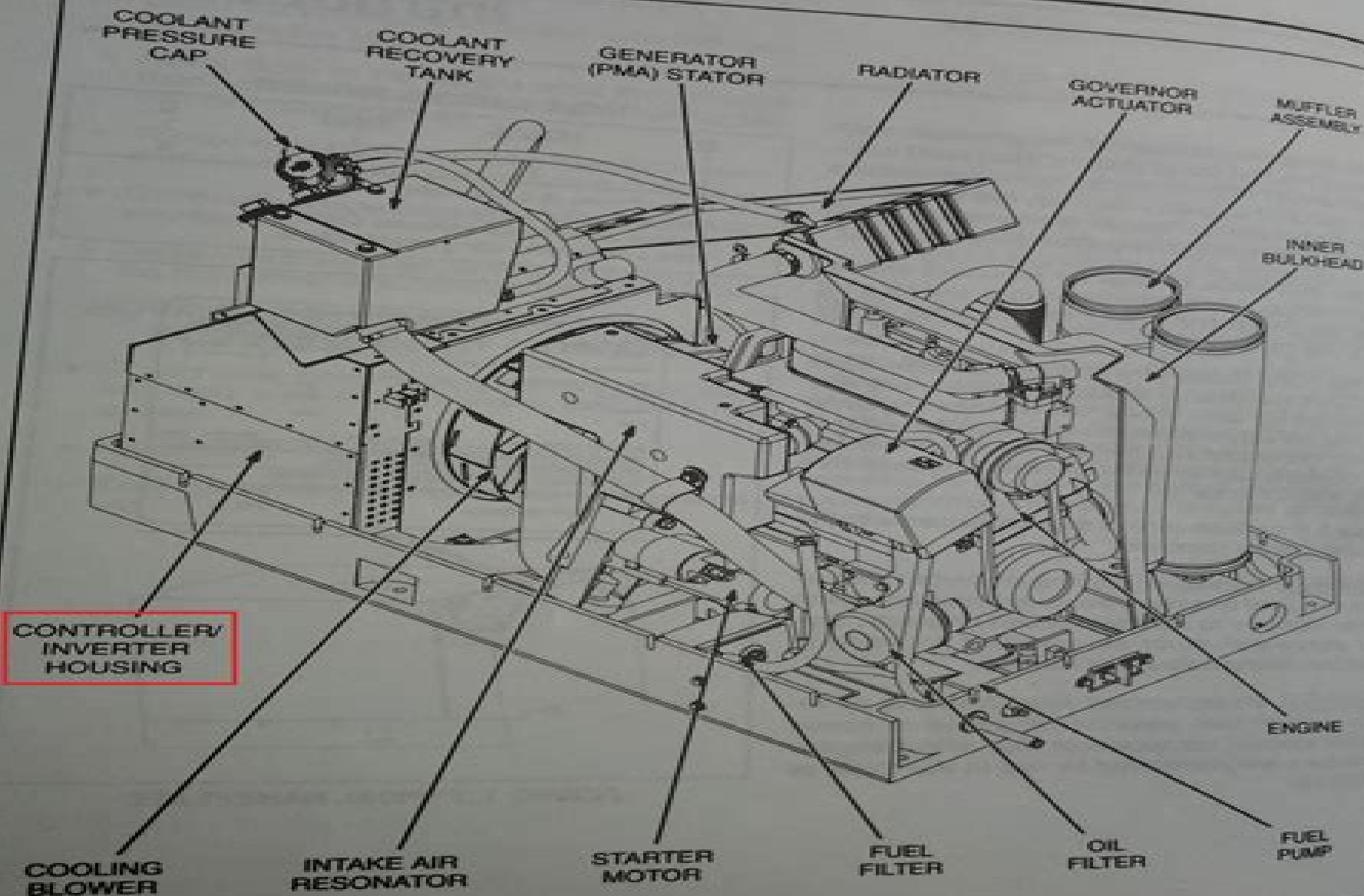
FIGURE 2. TYPICAL GENSET WITH HOUSING PANELS REMOVED
