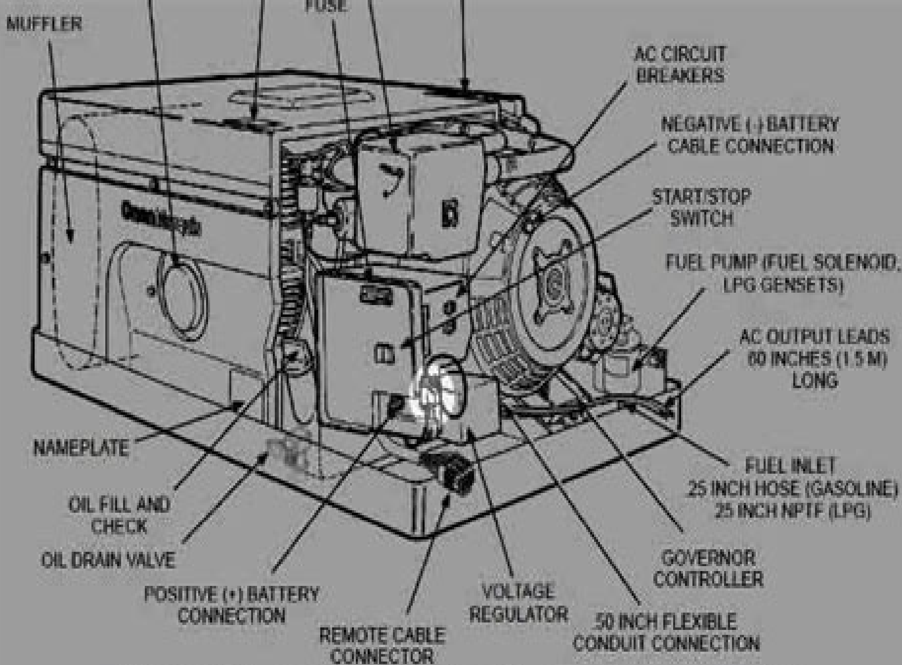
FIGURE 7-5. BOM/NHM GENERATOR SET (ELECTRONIC-GOVERNOR VERSION)
