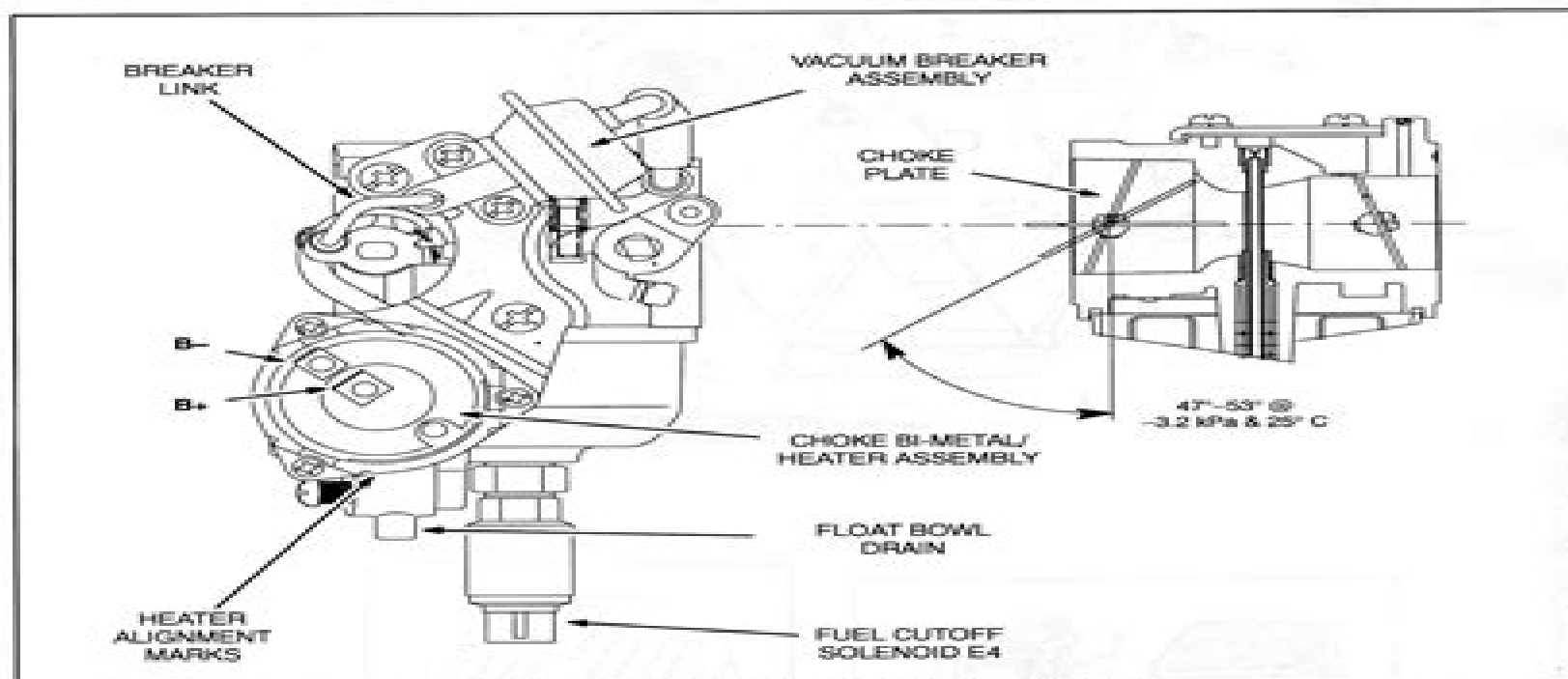
FIGURE 8-10. CARBURETOR / CHOKE ASSEMBLY
