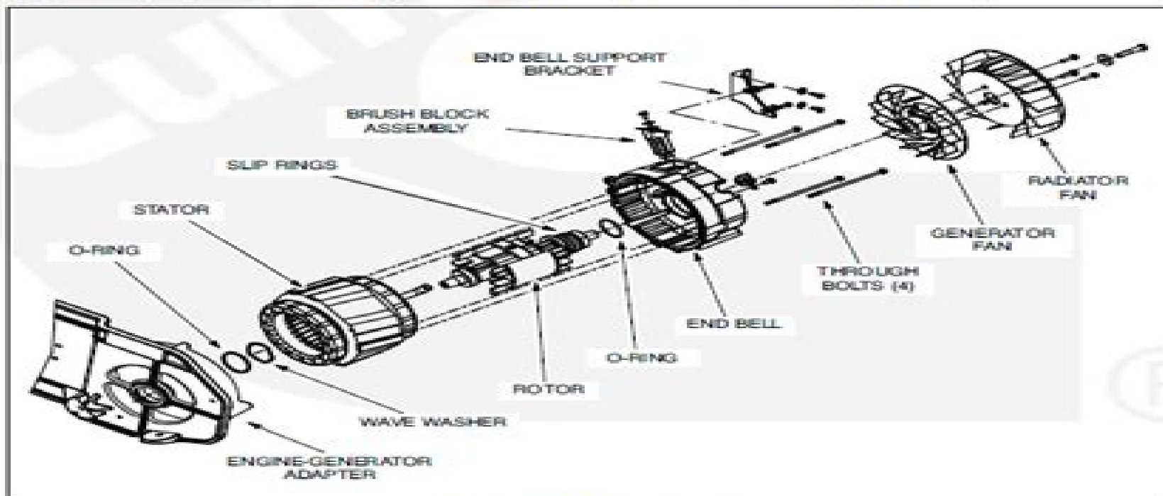
FIGURE 6-1. GENERATOR
