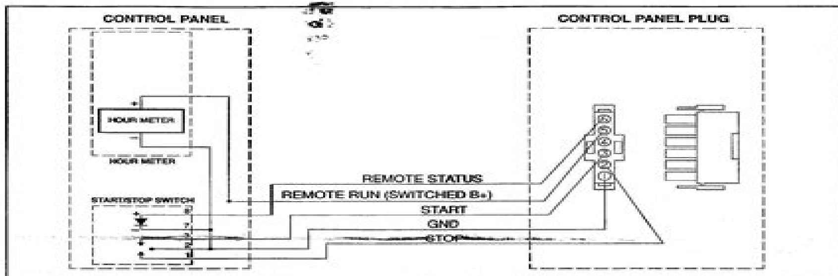
FIGURE 6. KIT 300-5332 REMOTE CONTROL WIRING DIAGRAM
