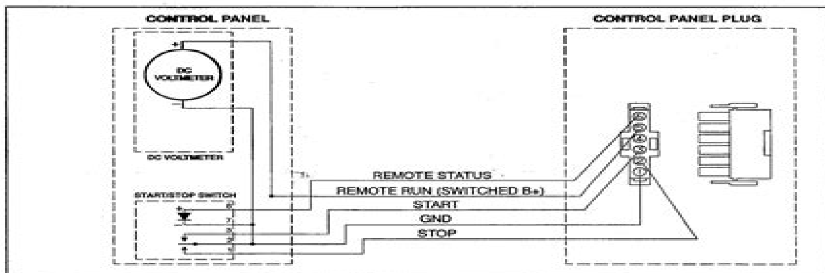
FIGURE 7. KIT 300-5333 REMOTE CONTROL WIRING DIAGRAM
