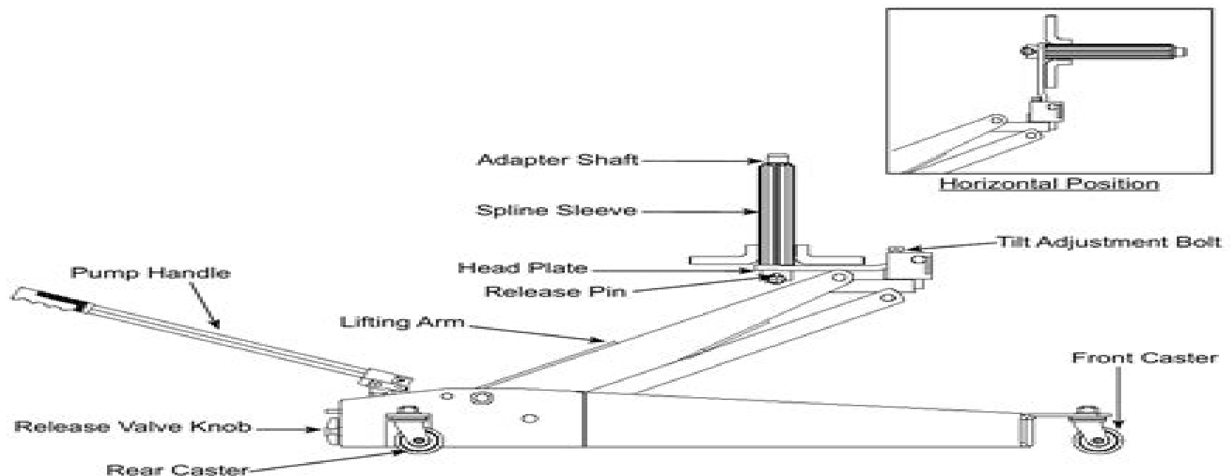
Figure 1 - Model 40500 Components
