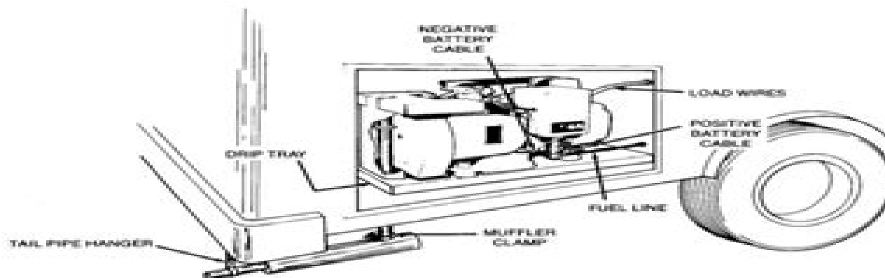
FIGURE 1. TYPICAL RV GENERATOR SET INSTALLATION
