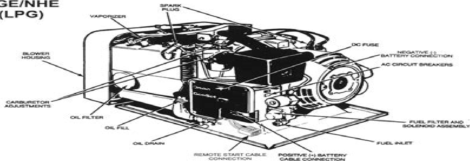
FIGURE S-1. TYPICAL EMERALD GENERATOR SETS
