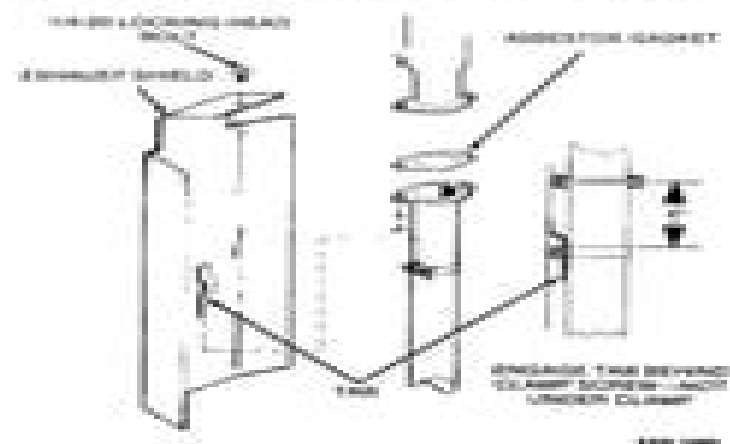
FIGURE 3. EXHAUST SHIELD TAB ENGAGEMENT
