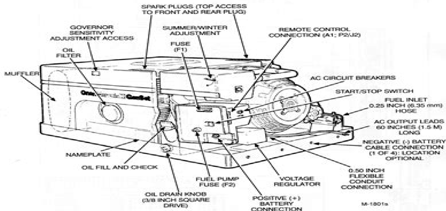
FIGURE 7-1. BGM/NHM GENERATOR SET (MECHANICAL-GOVERNOR VERSION)
