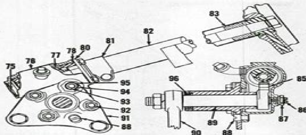
Fig. AC16—Gemmer steering gear assembly as used in early production B and C models.
