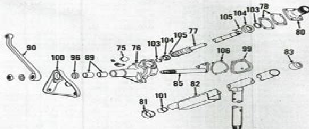
Fig. AC17—Ross steering gear assembly (exploded view) as used in later and current production B, C, and all CA tractor models.
