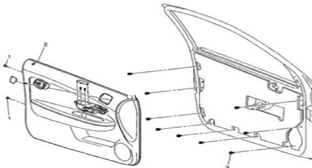
Fig. 2: Trim Panel Replacement - Side Front Door Courtesy of GENERAL MOTORS CORP.
