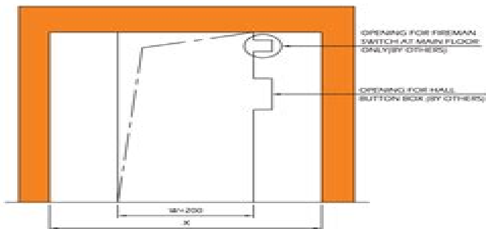
FRONT VIEW OF ENTRANCE
