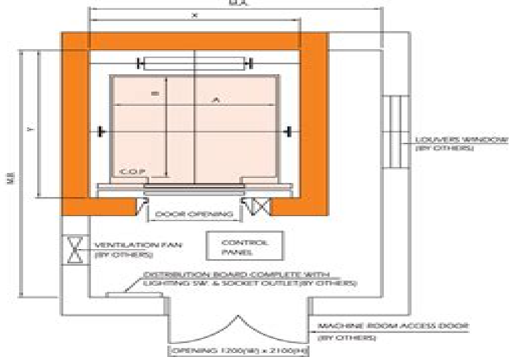
PLAN OF HOISTWAY & MACHINE ROOM
