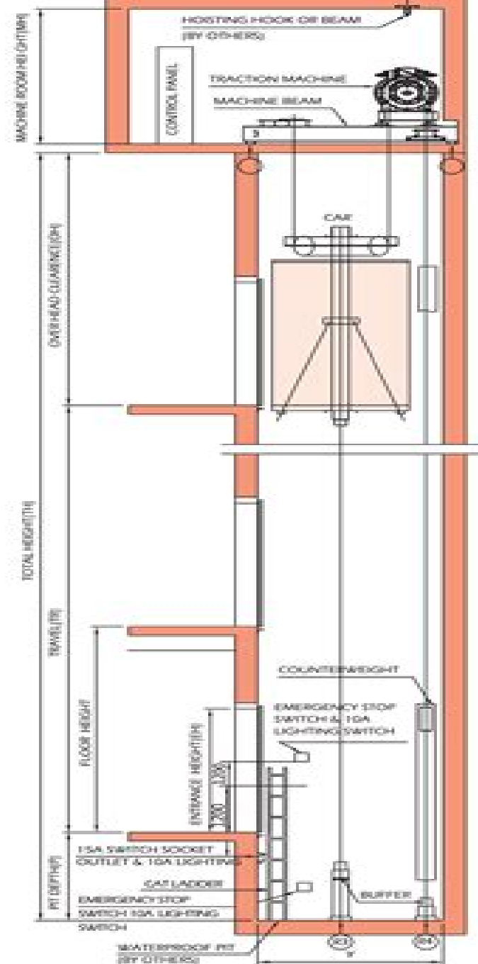
HOISTWAY SECTION
