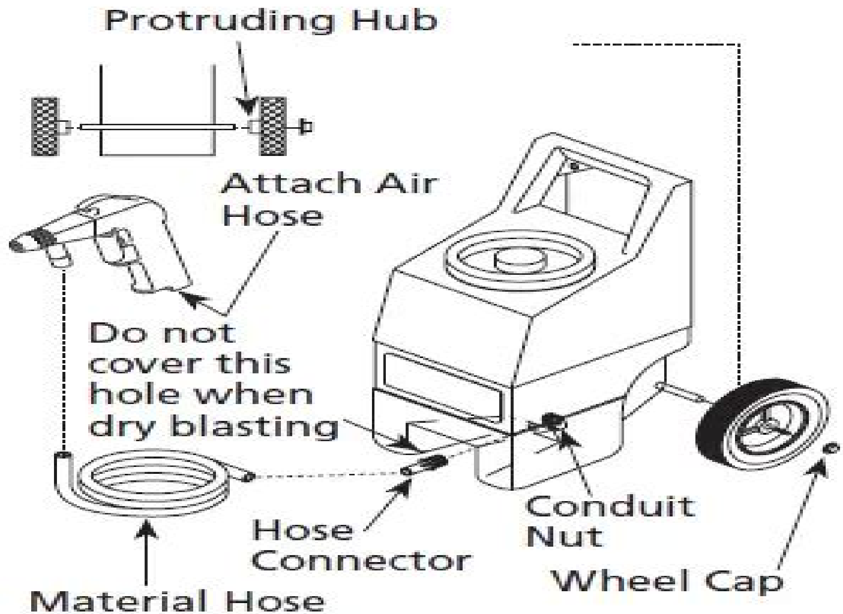
Figure 7 - Model AT121102
