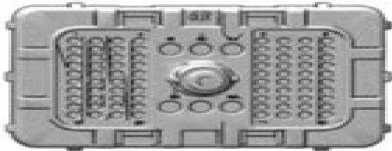
Illustration 1 Layout of the Connector Pins (view from the rear) g06060155
