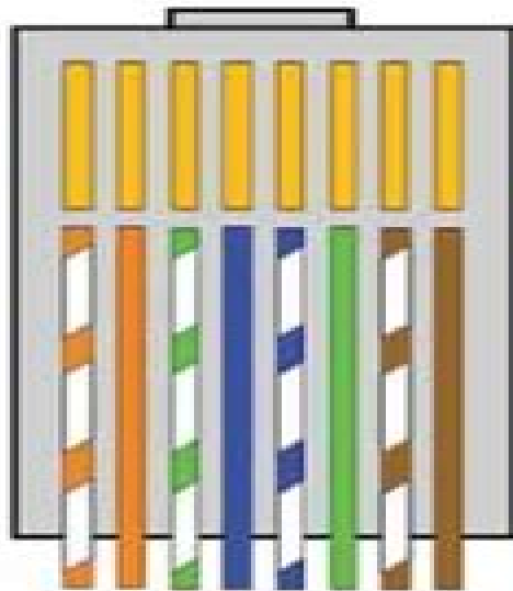
CAT5 Standard Patch Cord
