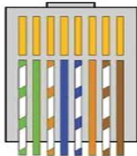
CAT5 Cross-over Cable
