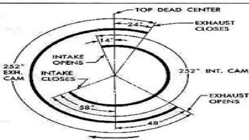
Fig. 6-48 Valve Timing Diagram for 3-Speed Synchro-Mesh
