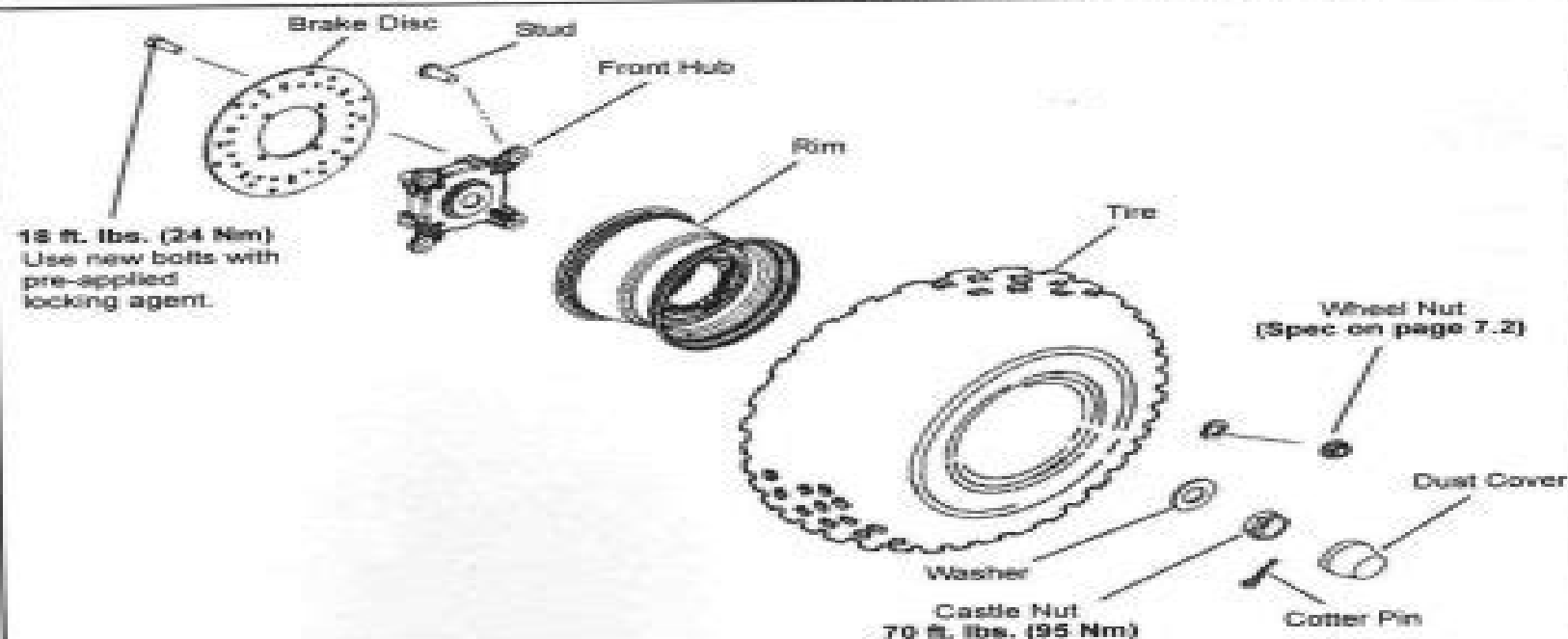
Front Hub/Wheel Exploded View
