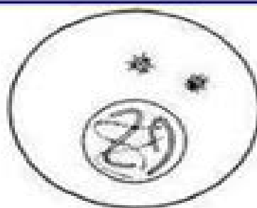
Prophase (early)
