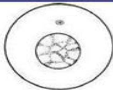
Interphase
