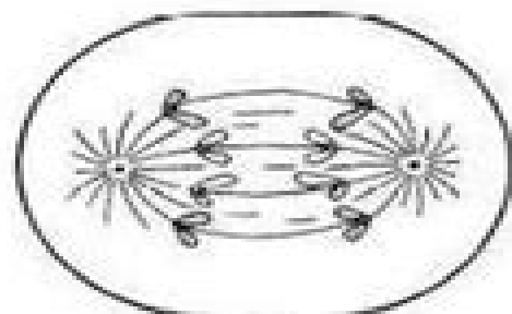
Anaphase
