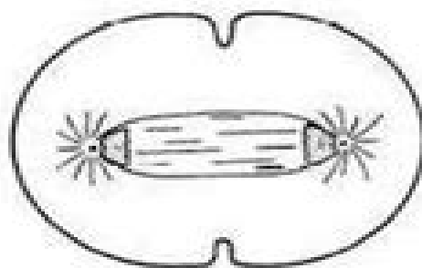
Telophase
