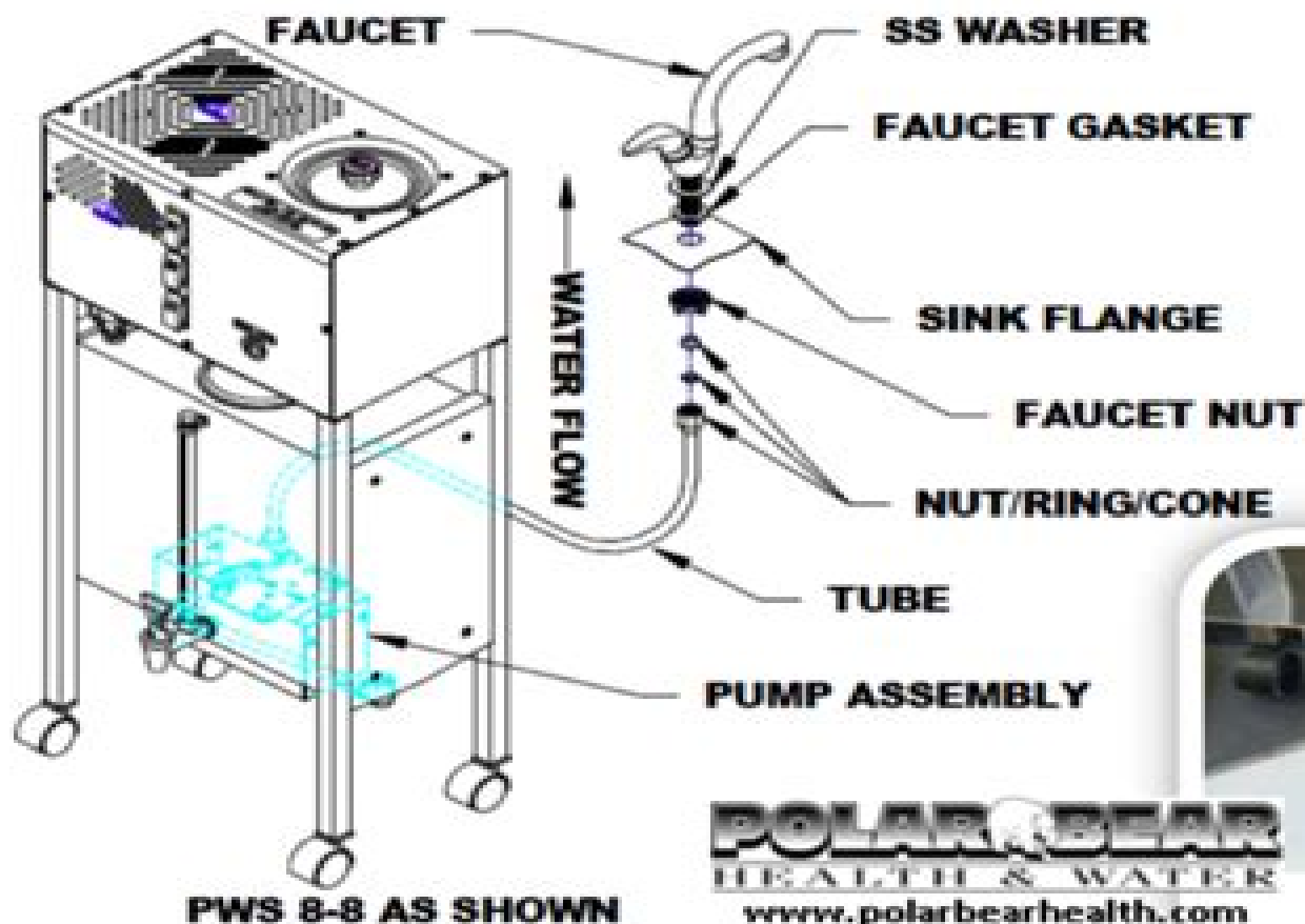
Pump Mounts Under Distiller's Storage Tank
