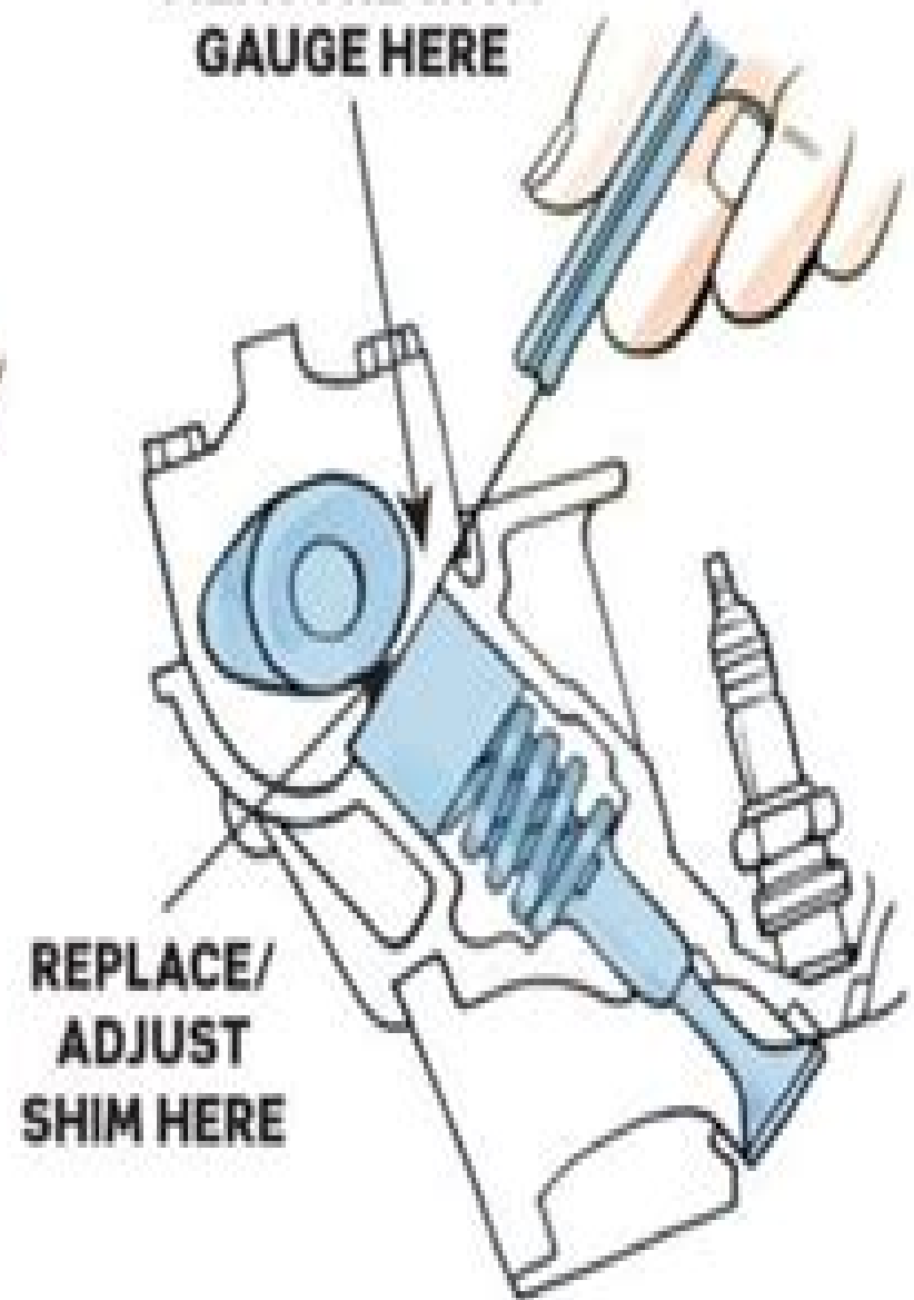
BUCKET-DRIVEN
