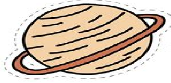
Saturn
