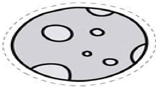
Mercury
