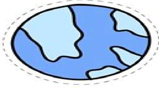
Neptune
