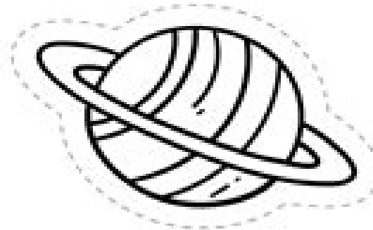
Saturn
