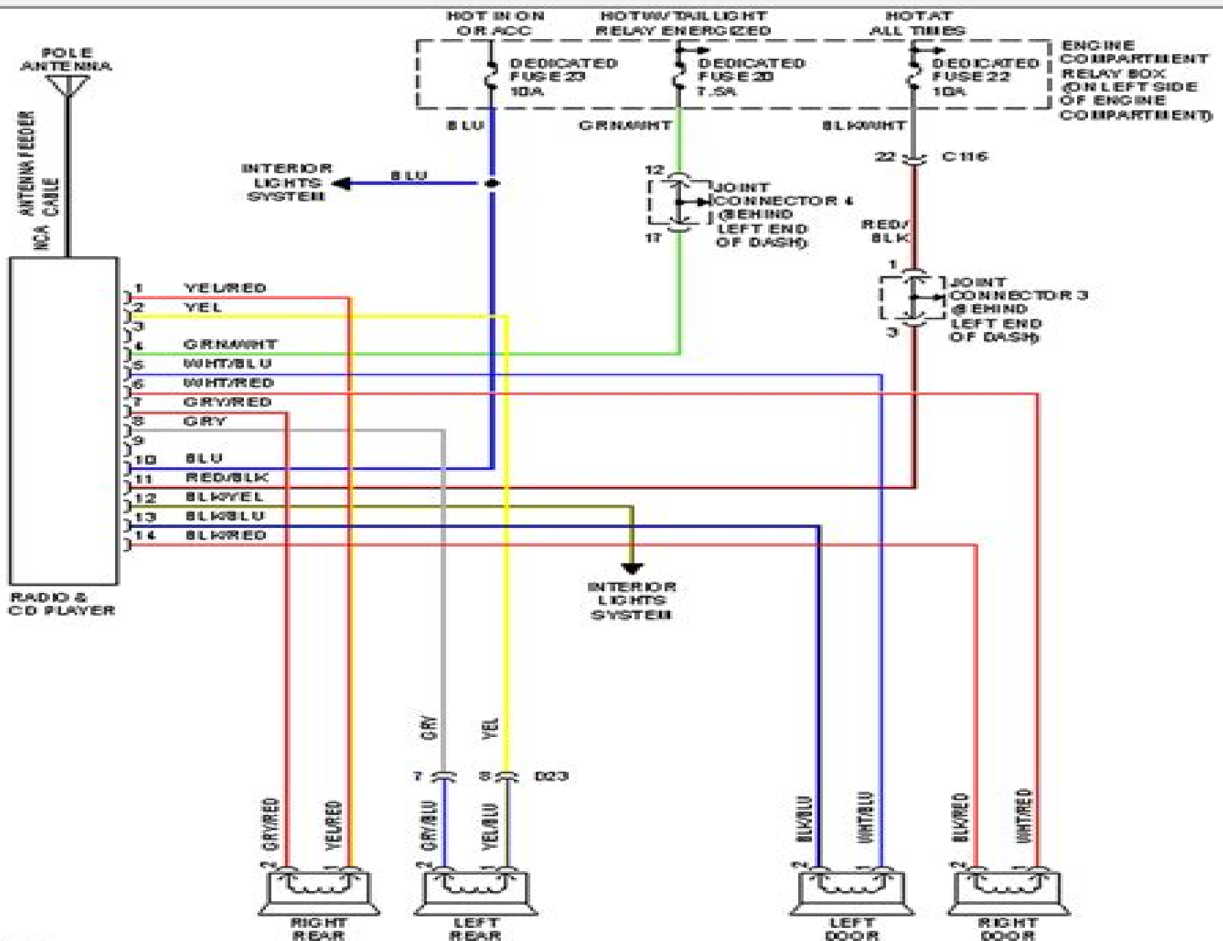
Fig. 39: Radio Circuit, W/O Amplifier
