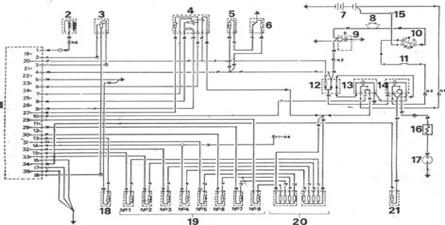
Fig 13.73 Supplementary wiring diagram for fuel injection system - 1982-84
