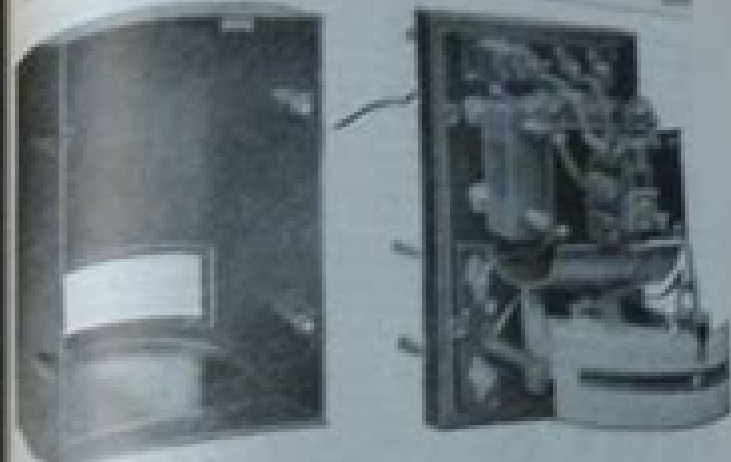
FIG. 22B.—Type TRD-A Temperature Indicating Relay: Left Front Cover Removed.
