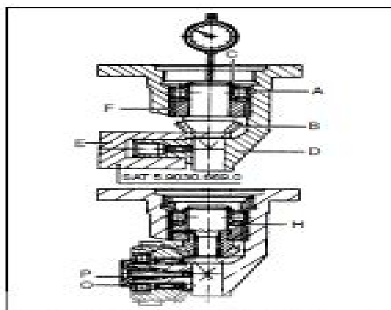
Fig. 17 - Installing pinion and crown gear.
