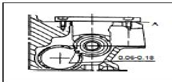
Fig. 19 - Installing engine governor control assembly into the cylinder block.
