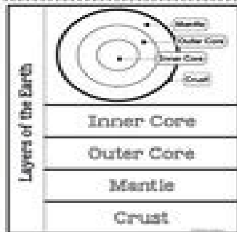
Layers of the Earth
